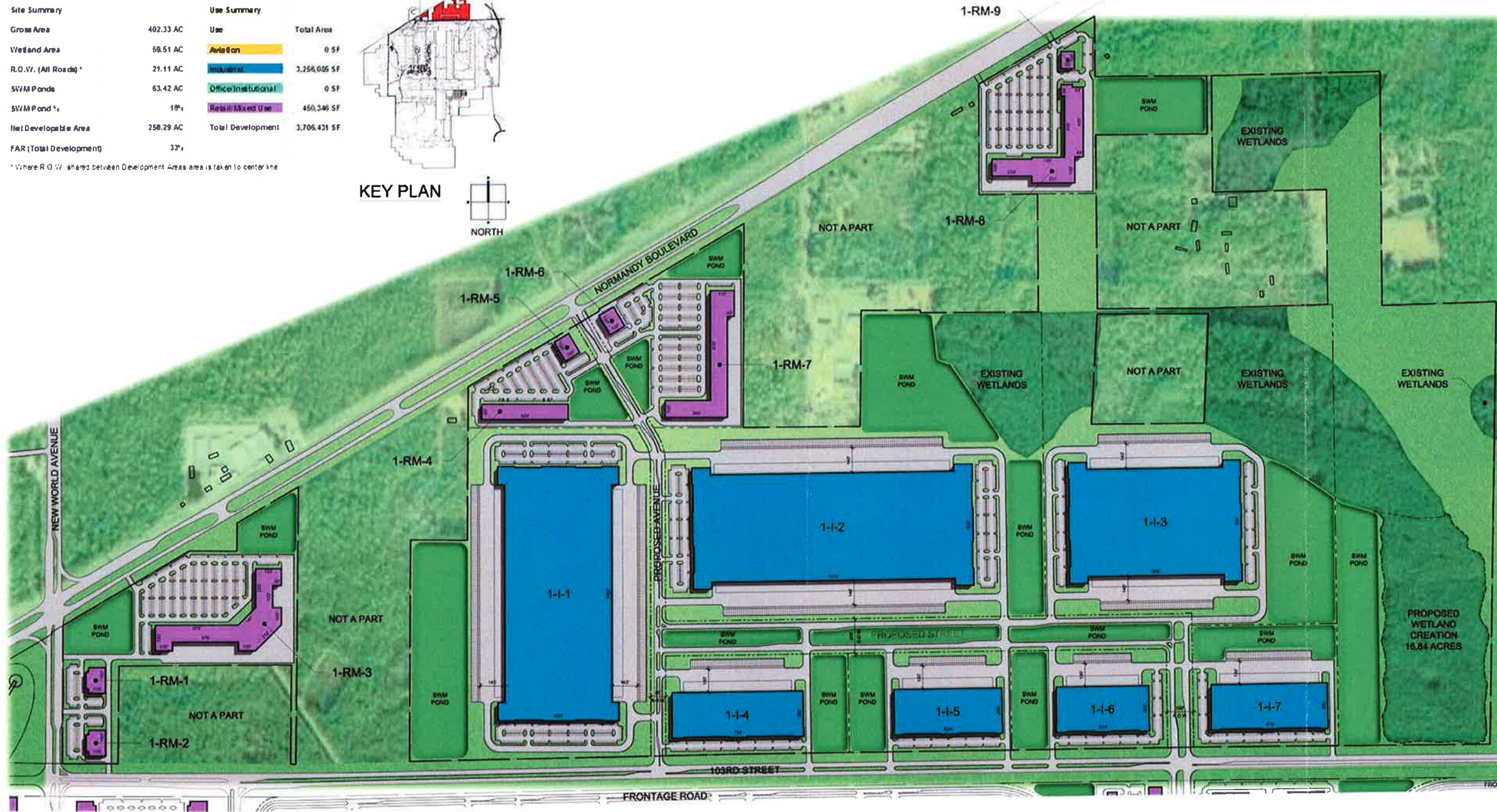
MASTER SITE PLAN - DEVELOPMENT AREA 1
